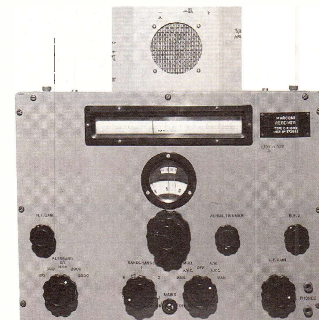
Marconi CR100 receiver as used by the Voluntary Interceptors.
