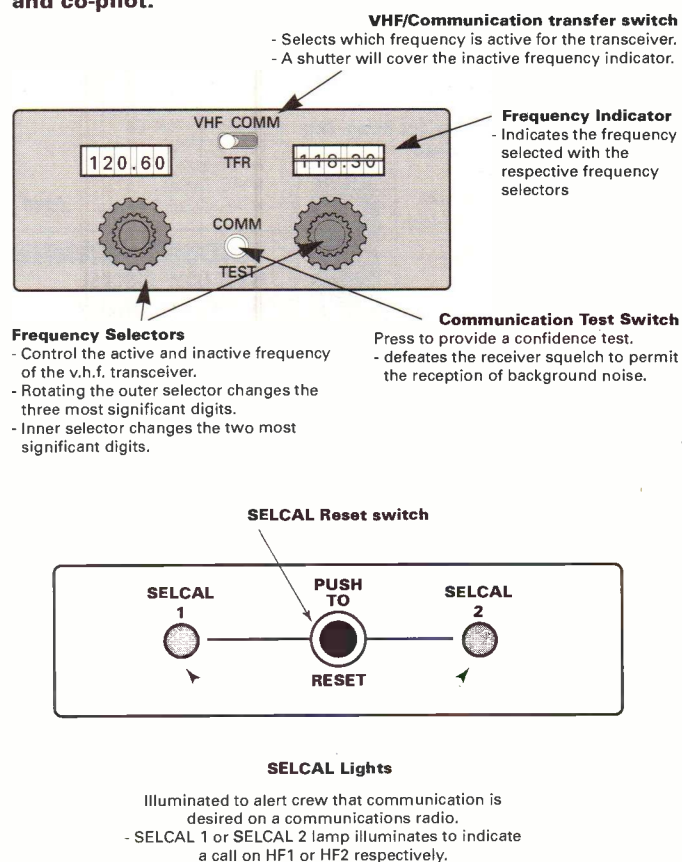
Fig. 2a: Selective Calling (SELCAL) visual warning as fitted in the forward electronic panel of BOEING 737/300.
