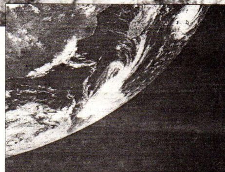
Fig. 1: NOAA picture from Geoffrey Chance.
