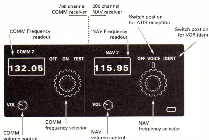
Fig. 1: Basic combined NAV/COM aircraft radio set.
